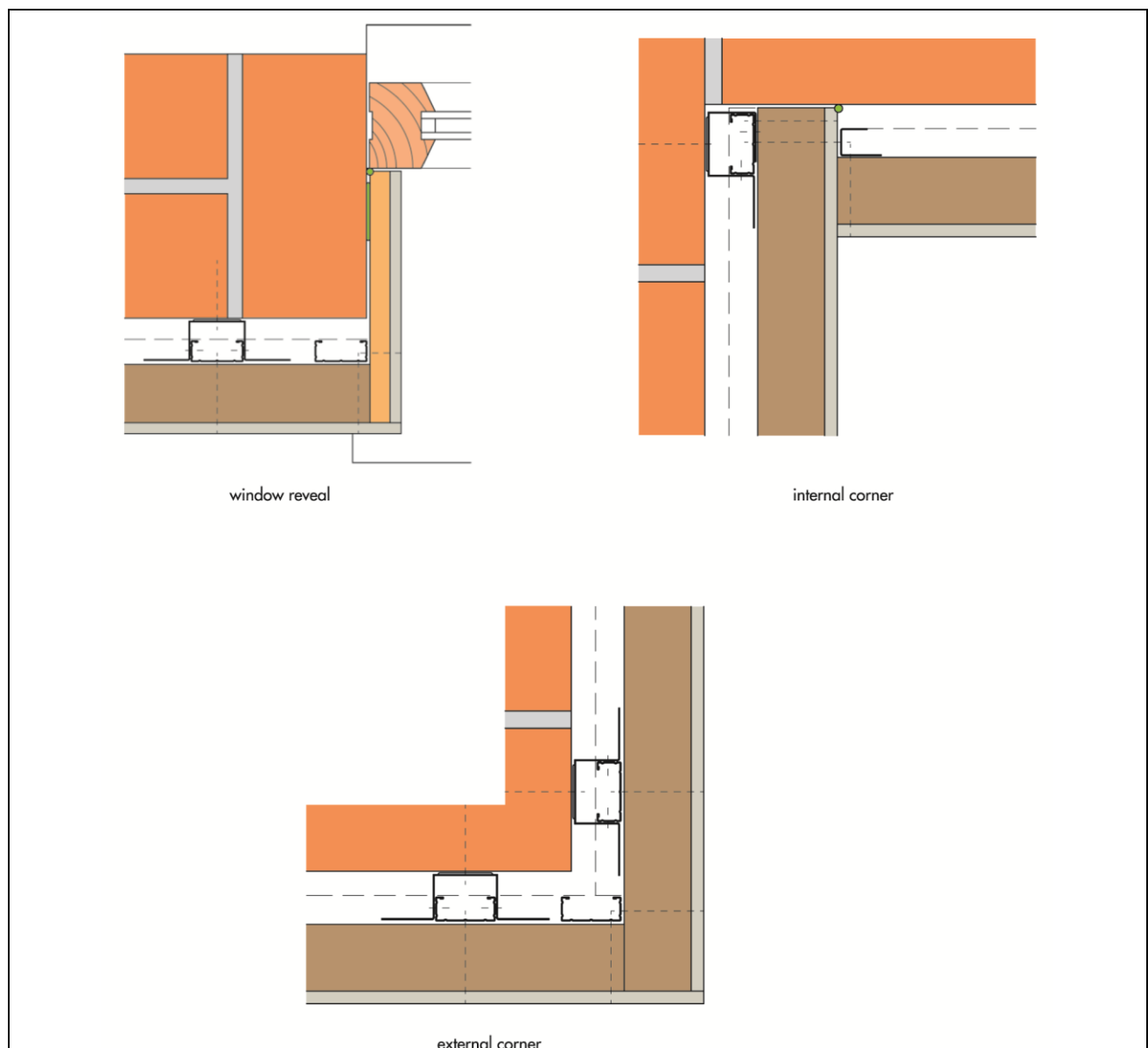
Figure 2 GypLyner UNIVERSAL construction details
