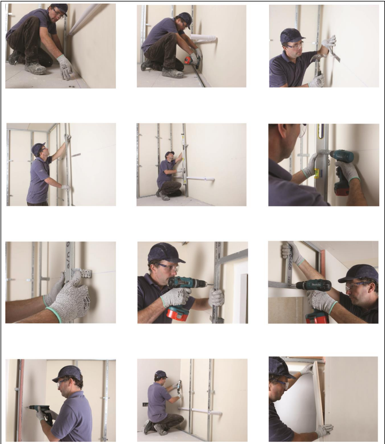
Figure 3 GypLyner UNIVERSAL installation details
