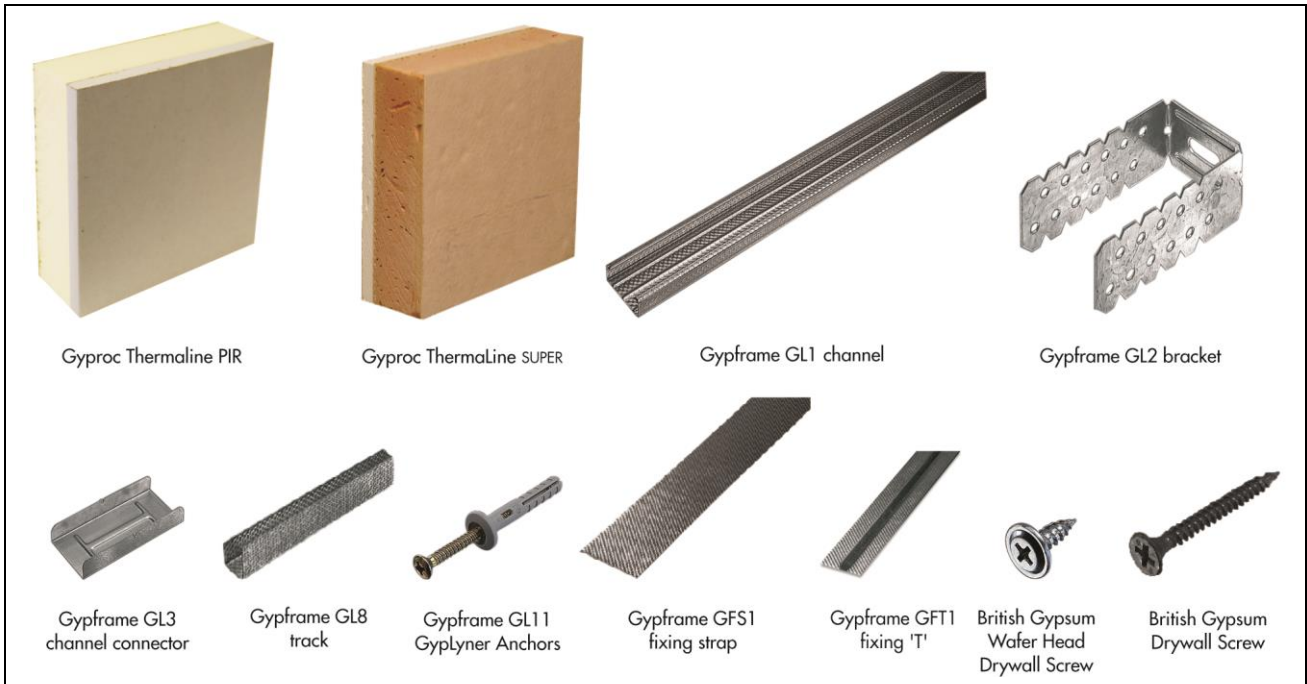
Figure 1 GyLyner UNIVERSAL — system components
